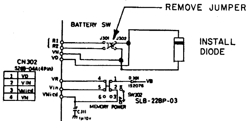
Figure 1. Memory PCB.
